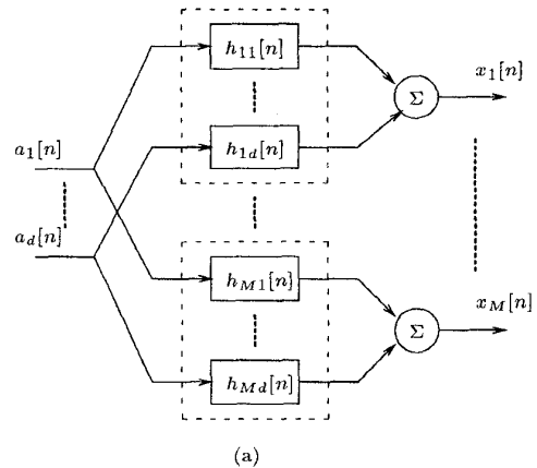
Fig. 1. Multiple-input and multiple-output channel
