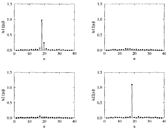
Fig. 6. The impulse response of the equalized system after 20,000 iterations
