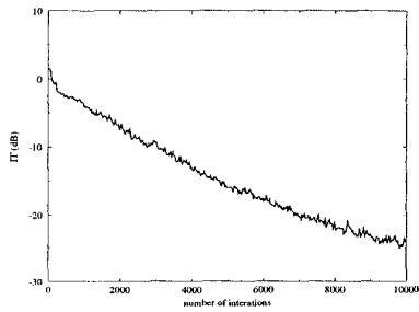
Fig. 5. Convergence of MIMO-CMA blind equalizer.
