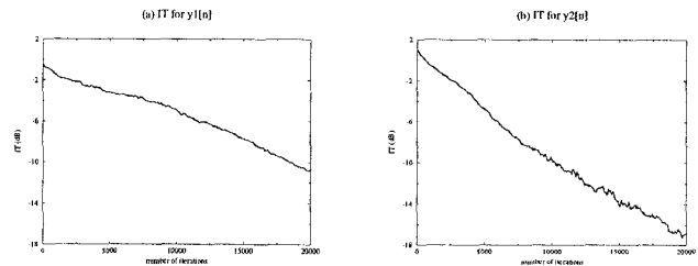
Fig. 7. Convergence of the new algorithm for the MIMO channel
