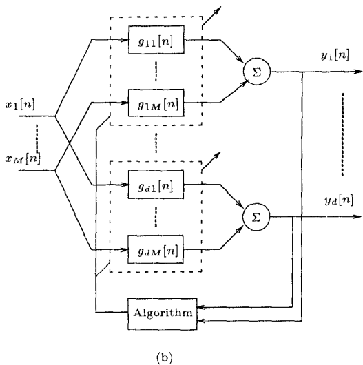
Fig. 2. Adaptive blind multiple-channel equalizer.
