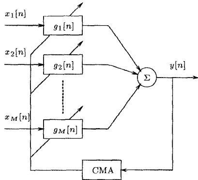
Fig. 3. The MIMO-CMA blind equalizer.
