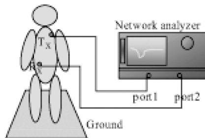
Fig. 1 Measuring system.
