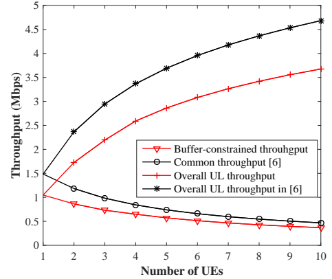
Fig. 11. Max-identical throughput varying with the number of UEs
