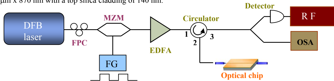
Figure 2 Experimental set-up for investigating on-chip SBS.
