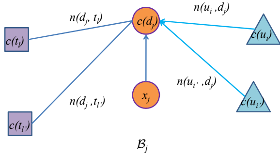
Figure 2: Illustration of the Markov blanket upon which c(d_j) is dependent.
