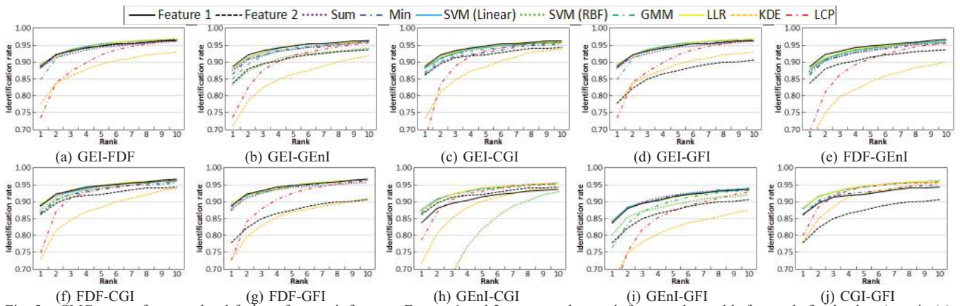
Fig. 5. CMC curves for score-level fusion of two gait features. Feature 1 and 2 corresponds to gait features denoted before and after hyphen (e.g., in (a), Feature 1 is GEI, Feature 2 is FDF). It can be said that the score-level fusion works well when the colored lines (fusion) are higher than both of the black lines (single features).
