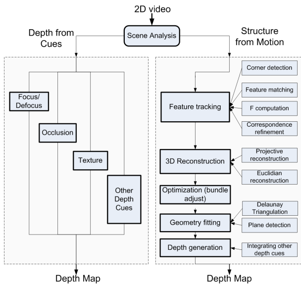
(a) Architecture for depth generation
