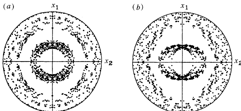
Figure 14. Calculated textures at the onset of necking for a latent hardening sheet ( q = 1.4 , n = 0.214 ) under balanced biaxial tension: (a) outside; and (b) inside the groove, with f = 0.997 and an initial texture shown in figure 2a.
