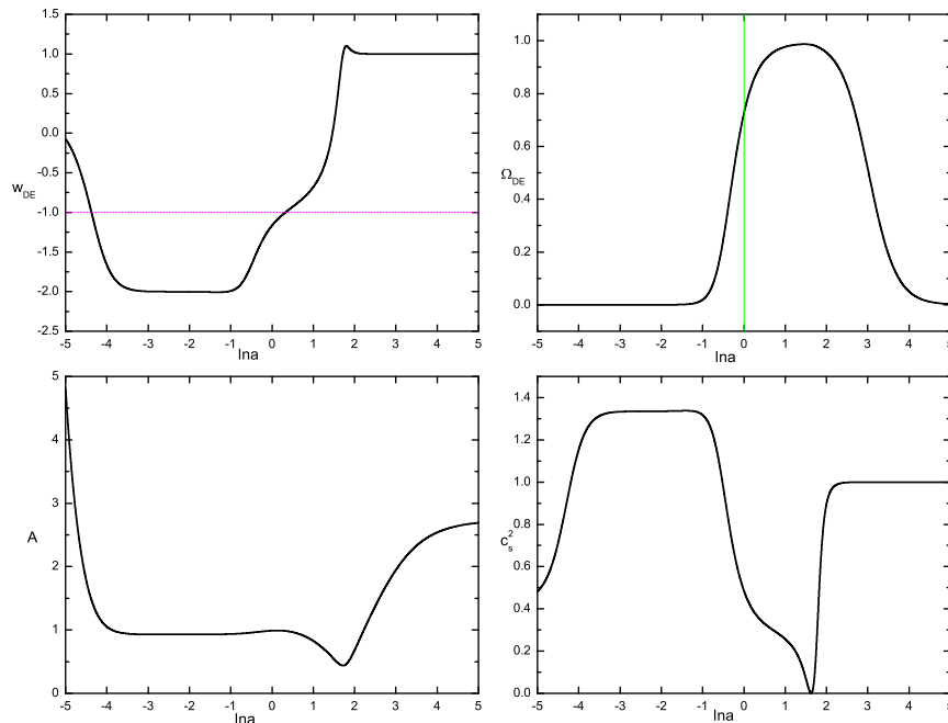
Figure 2. The equation of state w_{\text{DE}} , the energy density ratio \Omega_{\text{DE}} , parameter A and sound speed squared c_s^2 of dark energy of the model (5.10). The parameters are chosen to be c_1 = 3.0 \times 10^{122} , c_2 = 0.05 and the initial conditions are chosen in the far past when the universe was matter dominated. The equation of state crosses -1 recently, and becomes larger than 0 in the future. Both A and c_s^2 are positive during the evolution. The universe will be matter-dominant in the future.
