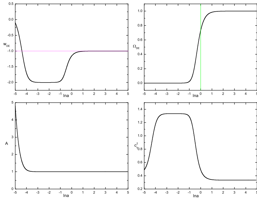
Figure 1. The equation of state w_{\text{DE}} , the energy density ratio \Omega_{\text{DE}} , parameter A and sound speed squared c_s^2 of dark energy of the model (5.10). The parameters are chosen to be c_1 = 3.0 \times 10^{122} , c_2 = 0 and the initial conditions are chosen in the far past when the universe was matter dominated. The equation of state crosses -1 recently, and approach to -1 in the future. Both A and c_s^2 are positive during the evolution. The universe will be dark energy dominant in the future.
