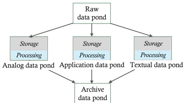
Fig. 2 Data flow in a pond architecture
