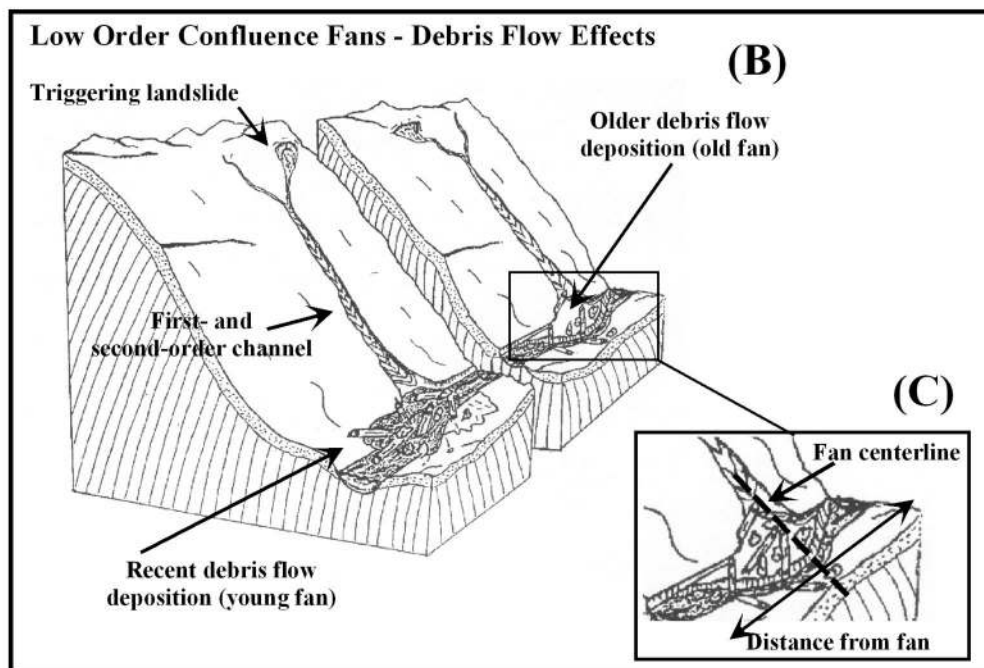
Figure 2. (A) Patterns of debris flow deposition in Harvey Creek basin. (A') White dots represent observed debris flow deposits (debris fans) at confluences of first- and second-order headwater streams observed in the field and predicted using the model of Benda and Cundy (1990). (A'') Dashed white lines show colluvial valley fill complexes where debris flows create semicontinuous deposits and terraces along upper third-order channels as modeled by Benda and Dunne (1997). (B) Effects of deposits depend, in part, on their age. (C) Morphological effects of debris flows were evaluated according to the distance from nearest (upstream or downstream) "fan centerline."
