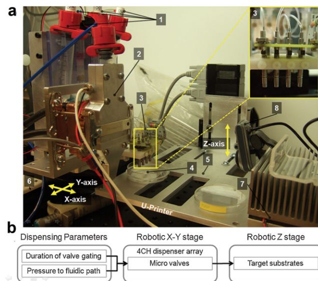
Figure 1. a: Picture of the 3D bio-printer platform shown with [1] a 4-channel syringe array as fluid cartridges for cells and hydrogel precursors, [2] independent heating/cooling unit for the dispenser, [3] a 4-channel dispenser array, [4] target substrate, [5] vertical stage, [6] horizontal stage, [7] vertical stage with heater/cooler, and [8] a webcam for monitoring of 3D printing process. Inset: close-up view of the 4-channel dispenser array. b: Schematics of dispensing operations of the 3D bio-printer. [Color figure can be seen in the online version of this article, available at www.interscience.wiley.com .]
