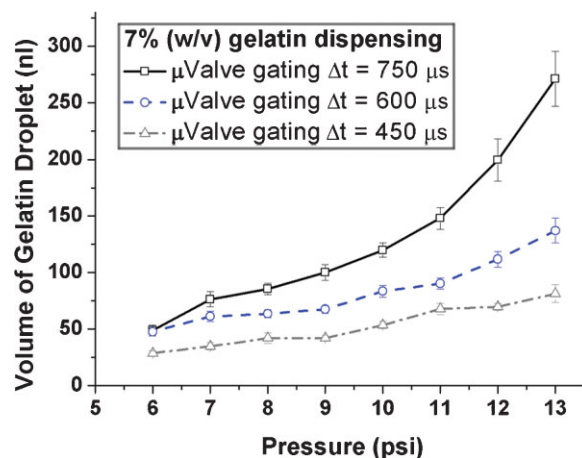
Figure 3. Mean droplet volume with standard error of 7% (w/v) gelatin solution ( n=8 ) with increasing pneumatic pressure to microvalve when the valve opening duration were 750, 600, and 450 μs. [Color figure can be seen in the online version of this article, available at www.interscience.wiley.com .]
