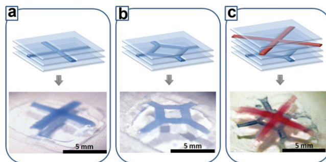
Figure 5. Three different designs of multi-layered collagen scaffold with fluidic channels (the upper row) and the actual constructions of those after gelatin removal using the bio-printer (the lower row). a: The printed “cross” pattern of the sacrificial gelatin was embedded in 2nd layer of three multi-layered collagen scaffold and selectively removed by warming and perfusion. PBS with blue-colored microspheres was injected into the gelatin removed fluidic channel (visualized in blue). b: The printed complicated “rotary” pattern of sacrificial gelatin was formed in 2nd layer of a three-layered collagen scaffold and selectively removed. Visualized in blue as in (a). c: Five multi-layered collagen scaffold with embedding and removal of sacrificial gelatin patterns was constructed as in Figure 2. Gelatin removed fluidic channel of rotary (blue, in 2nd collagen layer from bottom) and cross (red, in 4th collagen layer from bottom) patterns in collagen scaffold were visualized using PBS with colored microspheres. [Color figure can be seen in the online version of this article, available at www.interscience.wiley.com .]
