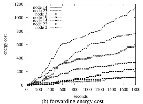
Figure 7: A network with 30 nodes running for 30 minutes with balance threshold.
