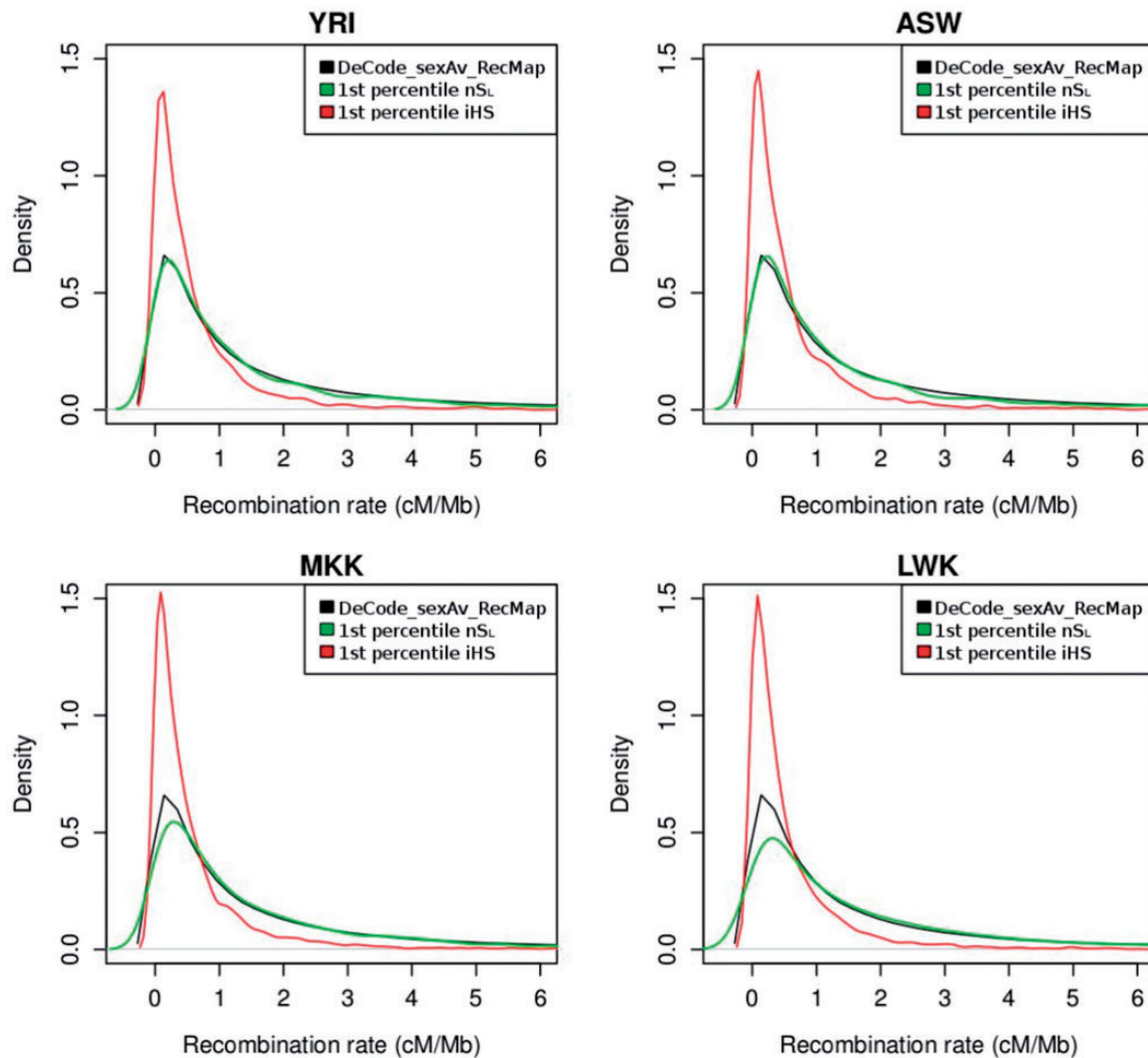
Fig. 4. Distribution of the recombination rate. Distribution of recombination rate for nS_L and iHS outliers (less than the first percentile of the respective empirical distributions). Recombination rate for nS_L outliers is shown in green, whereas recombination rate for the iHS outliers is in red. The distribution of the recombination rates for the entire genome is shown in black (data taken from the DeCode recombination map). Each panel in the figure corresponds to one HapMap3 population of African ancestry (YRI, ASW, MKK, and LWK).
