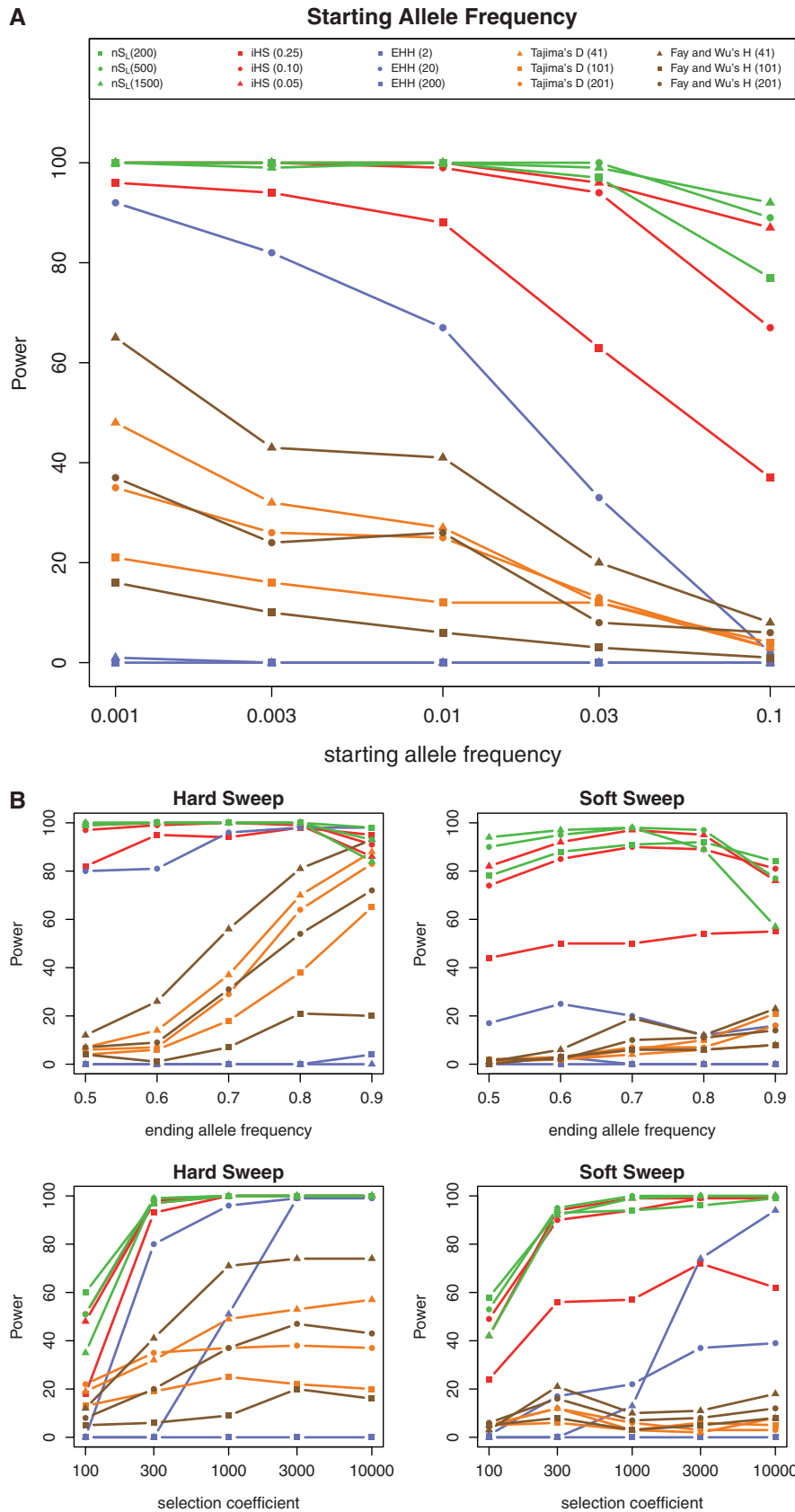
FIG. 2. (A) The power of five methods ( nS_L , iHS, EHH, Tajima's D, and Fay's and Wu's H ) for a range of starting allele frequencies (0.001–0.1). Power is defined as the proportion of simulations that reject the neutral null hypothesis at the 5% significance level. Each color corresponds to a method and symbols correspond to the window sizes used to run the methods (the specific window sizes used for the analysis are given in parenthesis). (B) The power of the five methods for a range of ending allele frequencies (0.5–0.9) (top two panels). The bottom two panels show the power of the methods for a range of selection coefficients ( 4N_s = 100 –10,000). The color scheme and symbols in these panels correspond to the legend embedded in (A).
