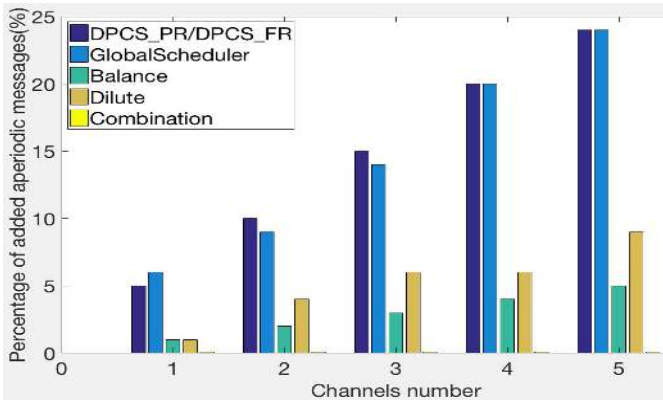
Fig. 4. Percentage of aperiodic messages transmitted over multichannel.
