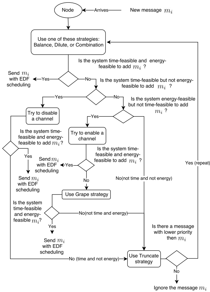
Fig. 1. Message scheduling global strategy for real-time RWSN under time and energy constraints.
