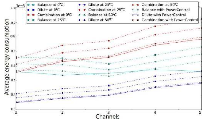
Fig. 7. Average energy consumption at transmission mode with using PowerControl strategy and without using it under three values of temperature \tau = 0^\circ\text{C} , \tau = 25^\circ\text{C} , and \tau = 50^\circ\text{C} .
