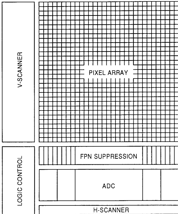
Fig. 13. Block diagram of an image sensor with FPN suppression and analog-to-digital conversion.
