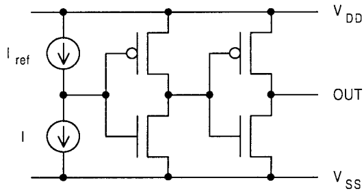
Fig. 10. Current comparator.
