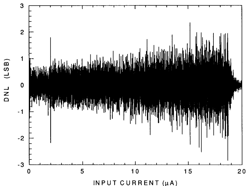
Fig. 11. Differential nonlinearity error for the 12-resolution operation.
