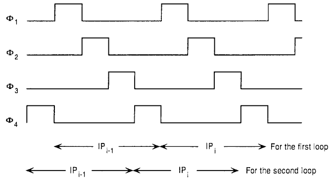
Fig. 7. Pulse timing diagram for the current-mode second-order incremental A/D converter.
