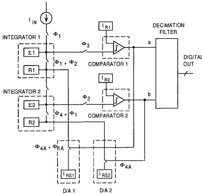
Fig. 6. Block diagram of the current-mode second-order incremental A/D converter.
