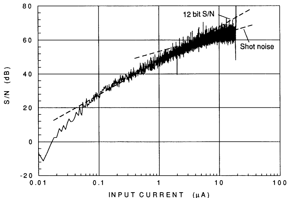
Fig. 12. S/N of the input current.
