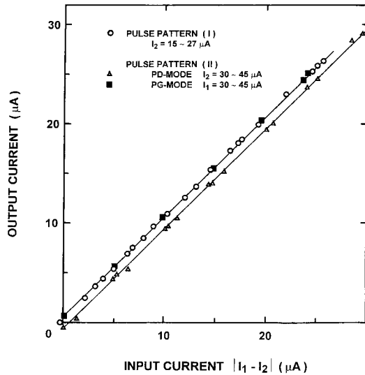
Fig. 4. Transfer characteristics of the FPN suppression circuit.
