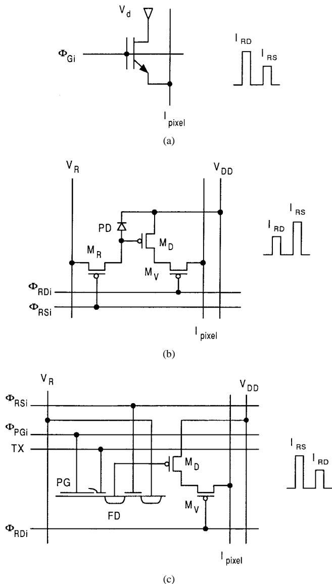
Fig. 1. Pixel configuration of current-mode APS's. (a) CMD pixel. (b) Photodiode (PD) CMOS APS pixel. (c) Photogate (PG) CMOS APS pixel.
