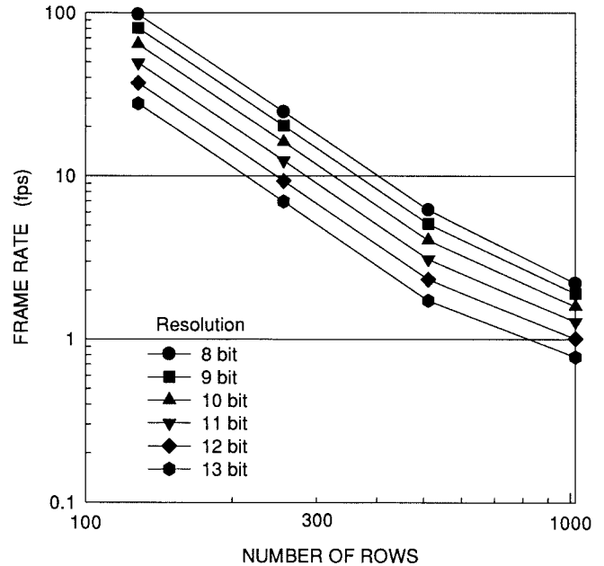
Fig. 14. Estimated relationship between frame rates and the number of rows.
