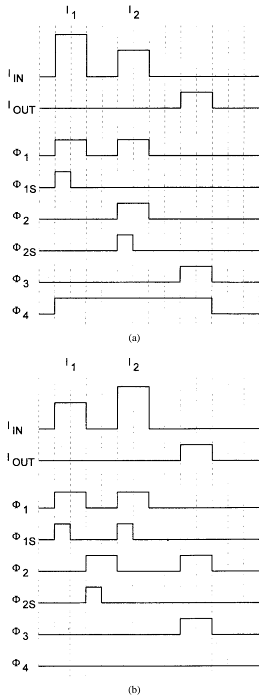
Fig. 3. Pulse timing for the new FPN suppression circuit. (a) Pulse pattern I, applicable for PG pixel and CMD pixel. (b) Pulse timing II, applicable for PD, PG, and CMD pixels.
