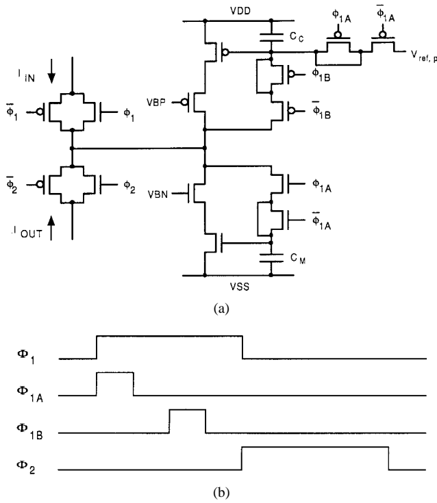
Fig. 8. Constant FeedThrough Current Copier Cell (CFTCCC). (a) Circuit configuration. (b) Pulse timing diagram.
