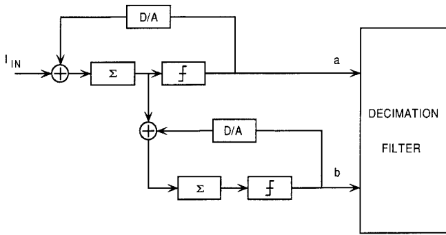
Fig. 5. Block diagram of the second-order incremental A/D converter.
