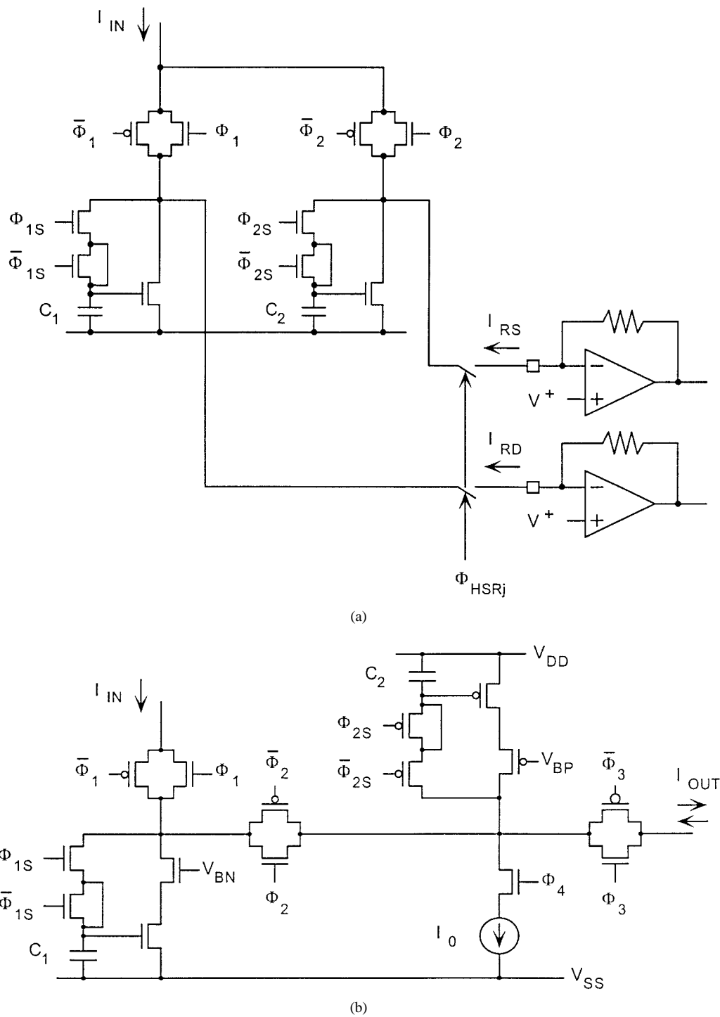
Fig. 2. Current-mode FPN suppression circuits. (a) FPN suppression circuit used in [12]. (b) New FPN suppression circuit.
