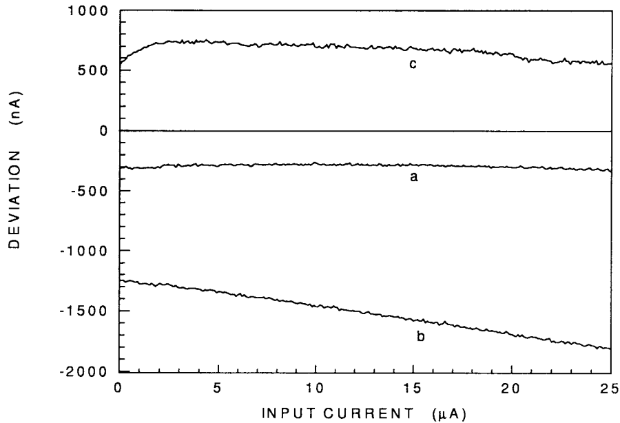
Fig. 9. Absolute error of an n -CFTCCC (a) with CFT operation V_{BP} = 2.25 V, V_{BN} = 2.75 V, (b) without cascoding V_{BP} = 0 V, V_{BN} = 5 V, (c) without CFT operation V_{BP} = 2.25 V, V_{BN} = 2.75 V.
