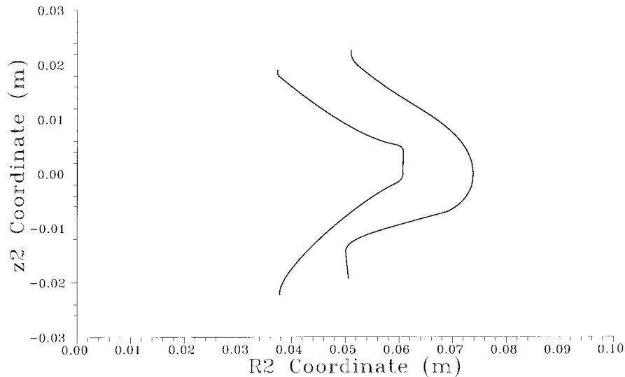
Fig. 6 Tool profiles generated from their given screw rotors
