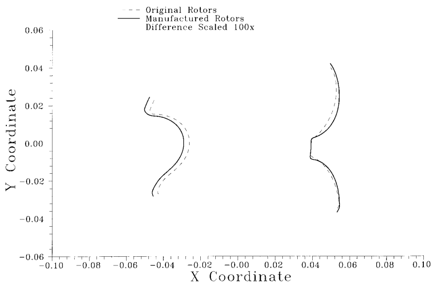
Fig. 7 Rotor profiles generated from a given tool
