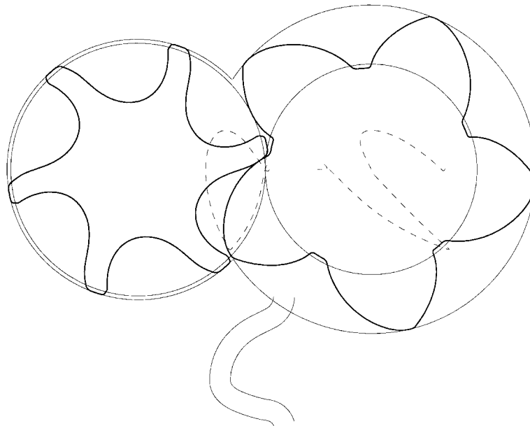
Fig. 4 'N' rotors in mesh, sealing line and clearance distribution
