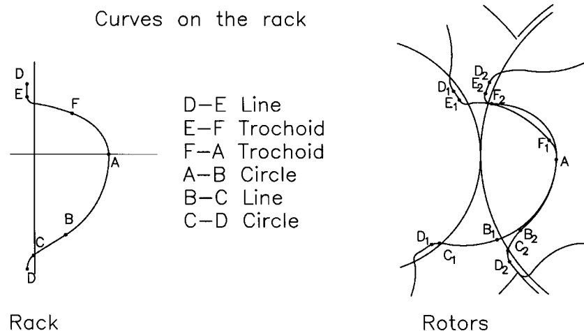
Fig. 3 'N' rack and rotor profile points
