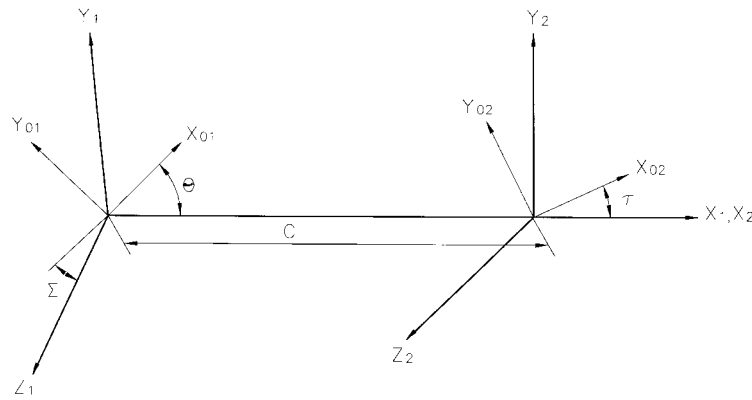
Fig. 2 Coordinate systems of crossed helical gears
