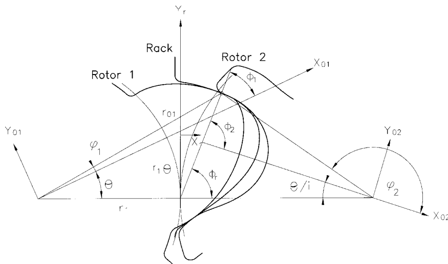
Fig. 5 Plane meshing of helical rotors
