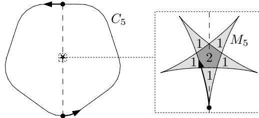
Fig. 8. The midpoint curve of a rounded pentagon, constructed analogously to C_{\Delta} of Figure 2, contains regions with winding number 2 and regions with winding number 1.
