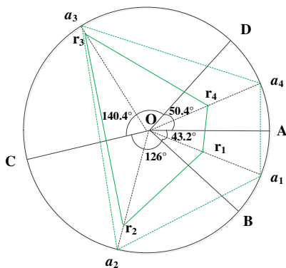
Figure 4. The radar chart of x_4
