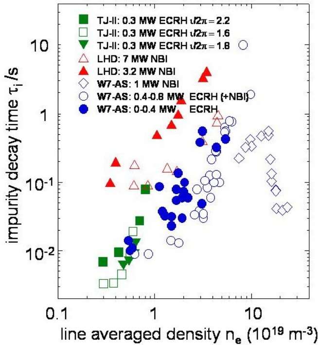
FIG. 1. Impurity confinement time vs. density in TJ-II, LHD, W7-AS. Open blue diamonds contain W7-AS HDH data. The data point at 10s should indicate no decay in W7-AS optimum confinement (OC) plasmas within the pulse duration.
