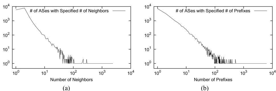
Fig. 4. Distribution of AS Neighbors and prefix assignments.
