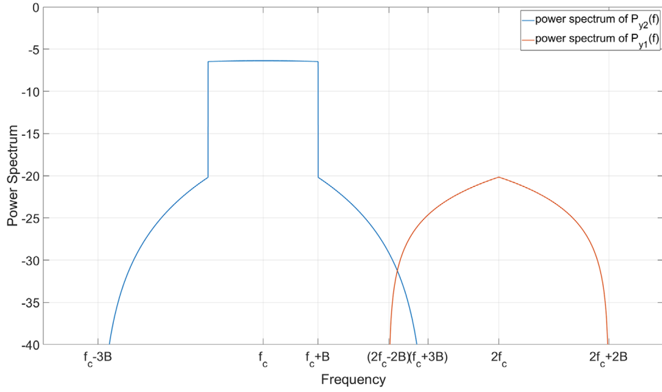
FIGURE 4 Power spectrum of P_{y_1}(f) and P_{y_2}(f) in scenario 2
