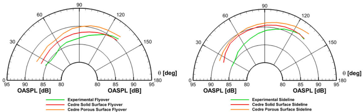
Figure 17. Overall sound pressure level integrated from 200 Hz to 5 kHz. Flyover results (left) and Sideline (right). Experimental results in green, solid surface analogy in red and porous surface results in orange.
