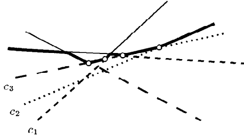
Fig. 3. The concave chains associated with the third level in an arrangement of lines. The level itself is drawn in bold; the dashed paths denote the concave chains c_1, c_2, c_3 ; and the circles denote the vertices of V_2 .
