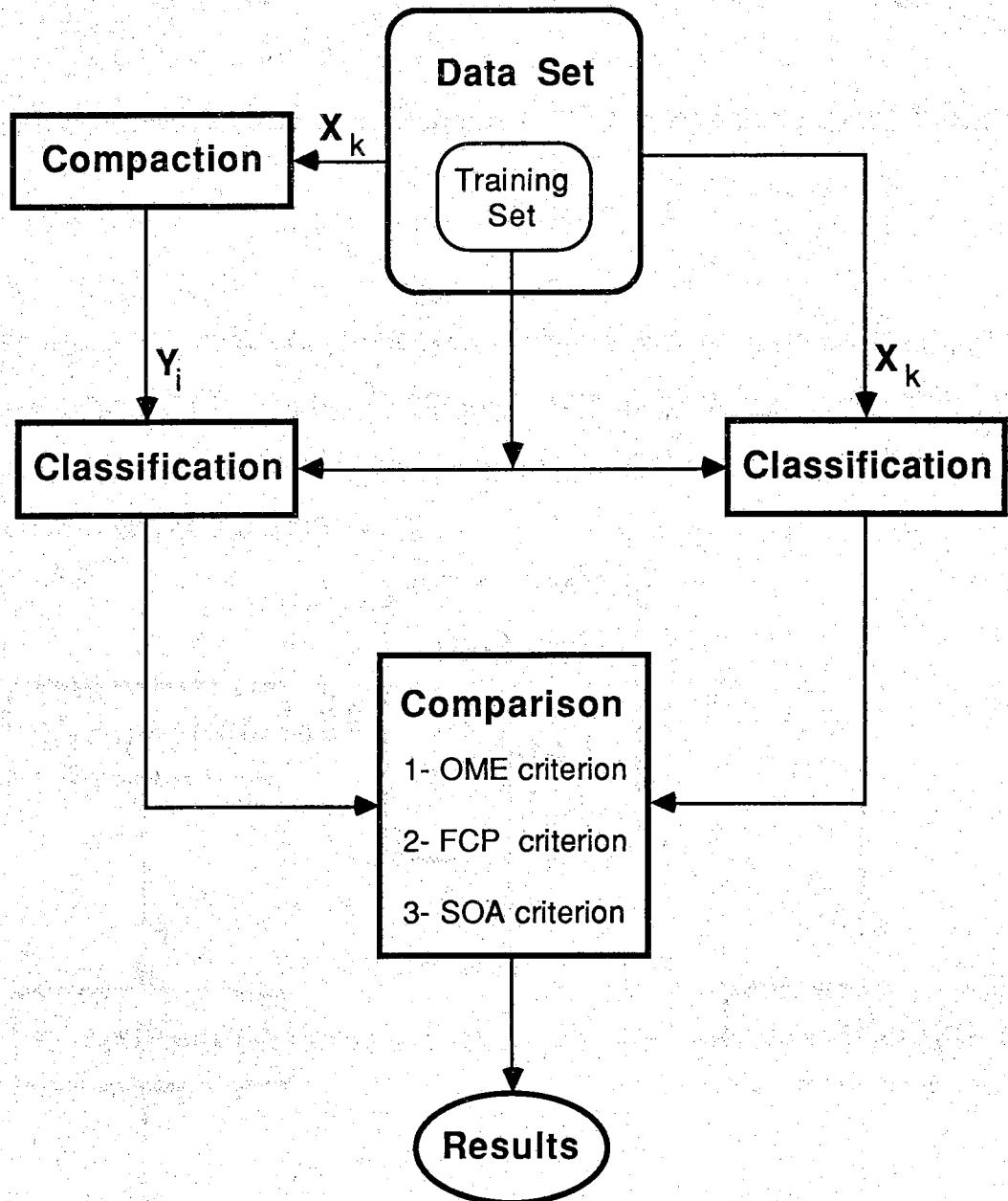
Fig. 4.1 Feature reliability evaluation
