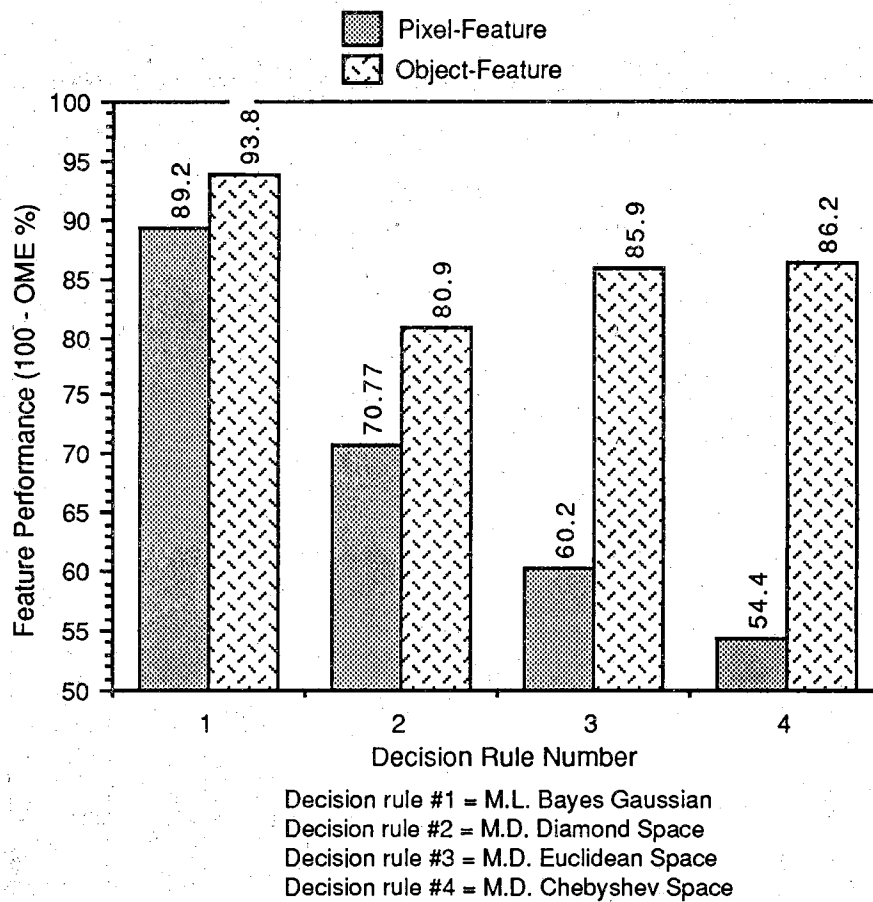
Fig. 4.7 Overall Feature Performance using different classification rules (data set No.1)
