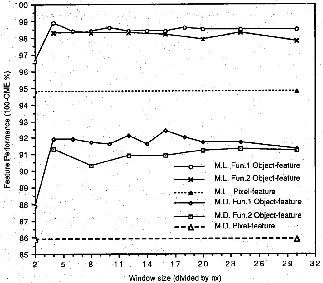
Fig. 4.5. Effect of window size on feature performance using data set No.2
