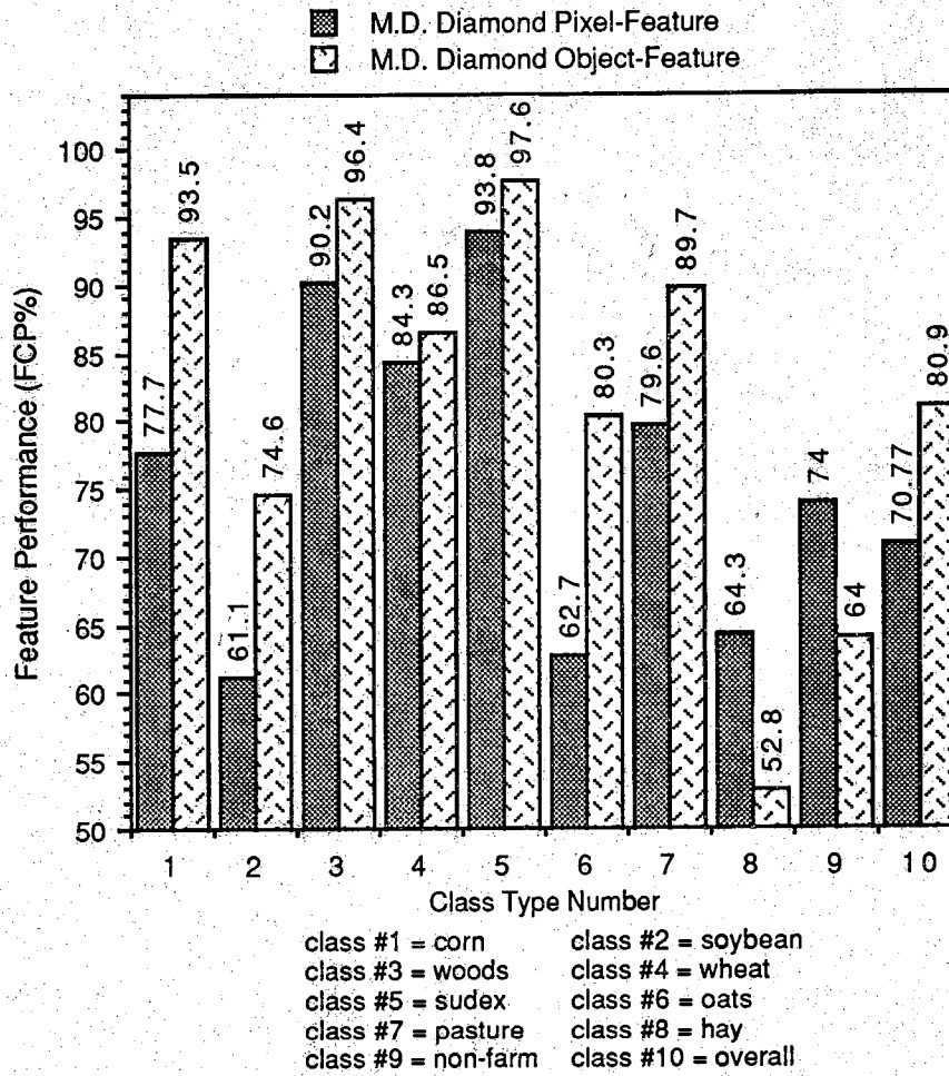
Fig. 4.10 Feature performance using M.D. Diamond space decision rule (data set No.1)
