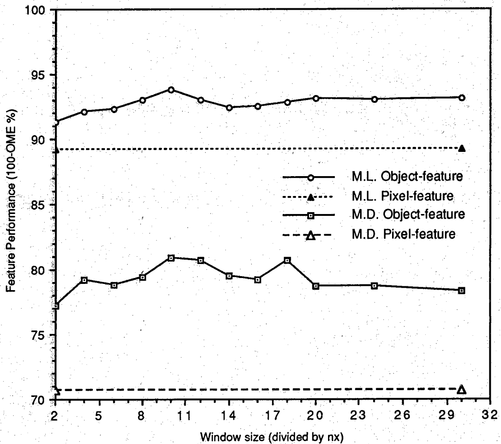
Fig. 4.4. Effect of window size on feature performance using data set No.1
