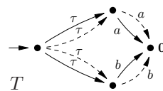
Fig. 5. All implementations of T have \tau -transitions.
