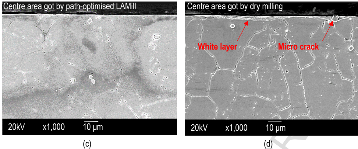
Fig. 18 Microstructure of path-optimised LAMill and dry milling subsurface: at edge area gotten by path-optimised LAMill (a) and dry milling (b), at center area gotten by path-optimised LAMill (c) and dry milling (d)
