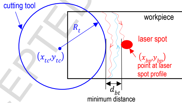
Fig. 6 Illustration of the safe distance between laser spot and cutting tool from top view during laser scanning
