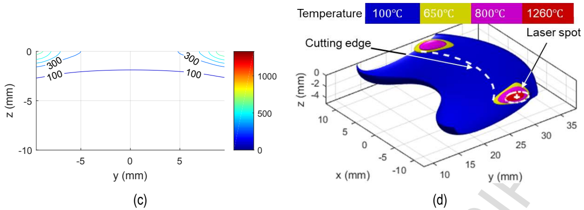
Fig. 4 Predicted temperature distribution for the initially chosen laser trajectory: on the top surface (a), on the depth of cut plane (b), along the cutting cross section(c) and the 3D view (d). Parameters used were: cutting width=19mm, cutting depth=0.26mm, feed rate=948mm/min (0.5mm/tooth) and laser beam diameter=3mm.
