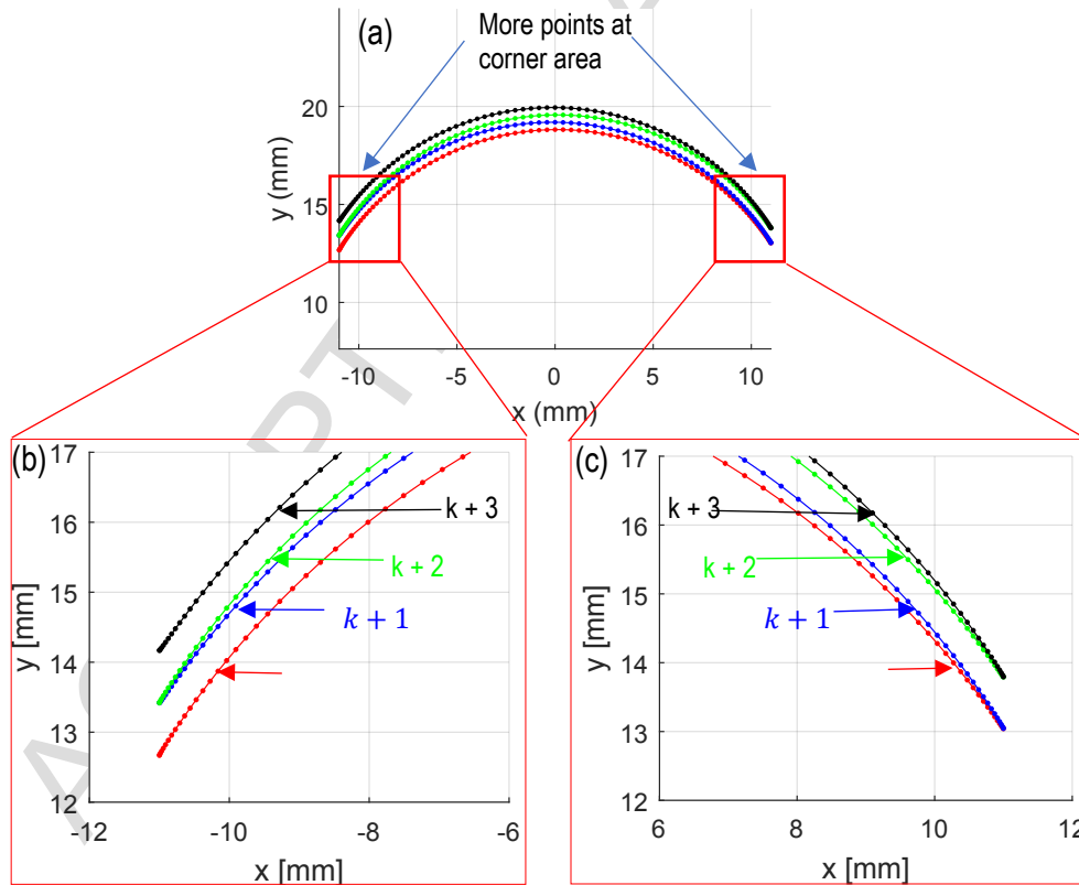
Fig. 2 Inverse problem with predefined laser trajectory for speed optimization: laser scanning path (a) and enlarged view at left corner (b) and right corner (c) area for k^{th} to (k+3)^{th} scanning
