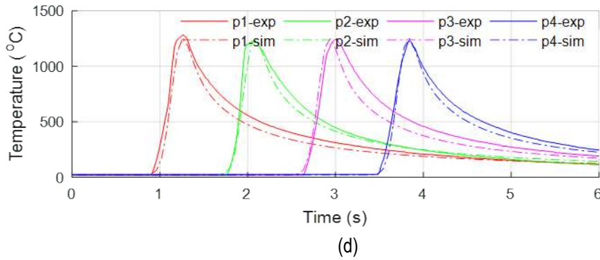
Fig. 10 Experiment results on direct problem for linear laser path scanning: measured (a) and simulated (b) temperature on the top surface, photo of the sample surface (c) and comparison between experimental (exp) and simulated (sim) temperatures at four selected points (P1~P4) (d)
