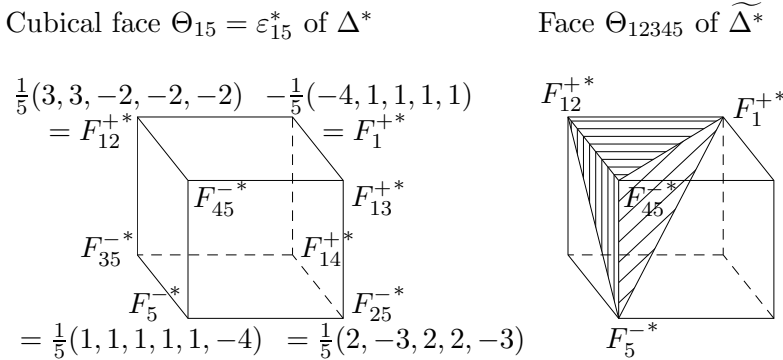
Figure 3: Three dimensional faces of \Delta^* and \widetilde{\Delta}^* .
