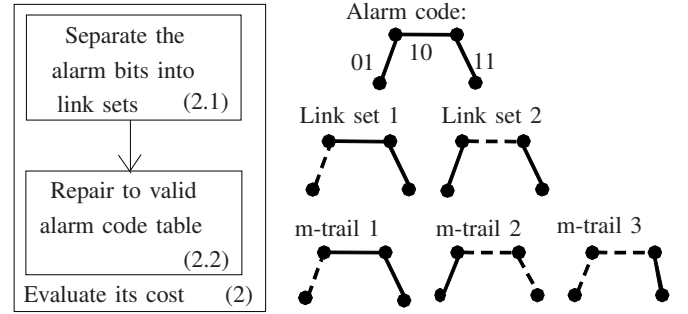
Fig. 6. An illustration of the cost evaluation method of an alarm code table of the 4 node line graph.
