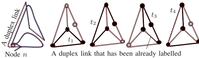
Fig. 4. The m-trails based on the close trail decomposition of a graph.
