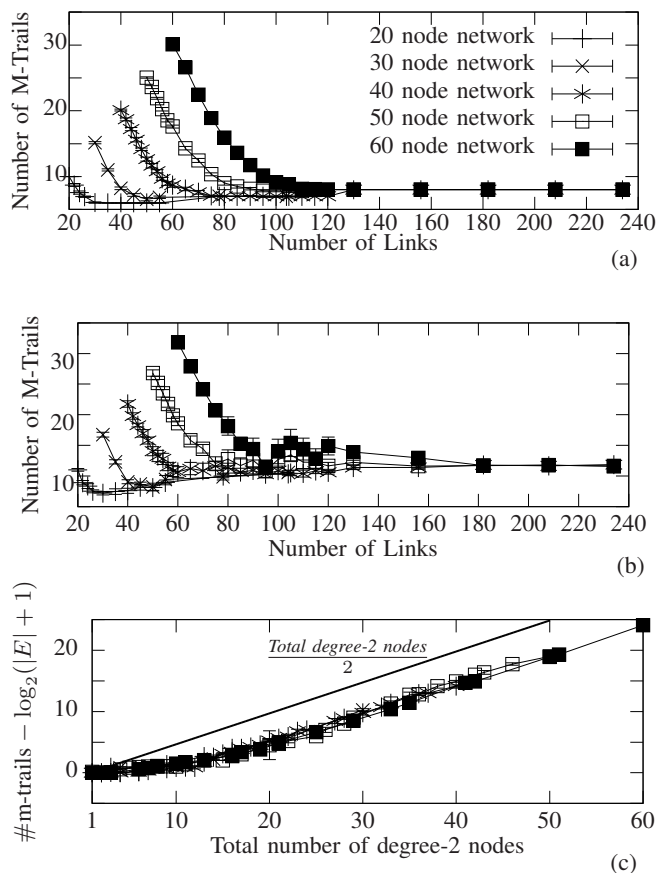
Fig. 10. The length of alarm code versus the number of added links for topologies of 20, 30, 40, 50, and 60 nodes. (a) \gamma = 1000 and (b) \gamma = 5 .
