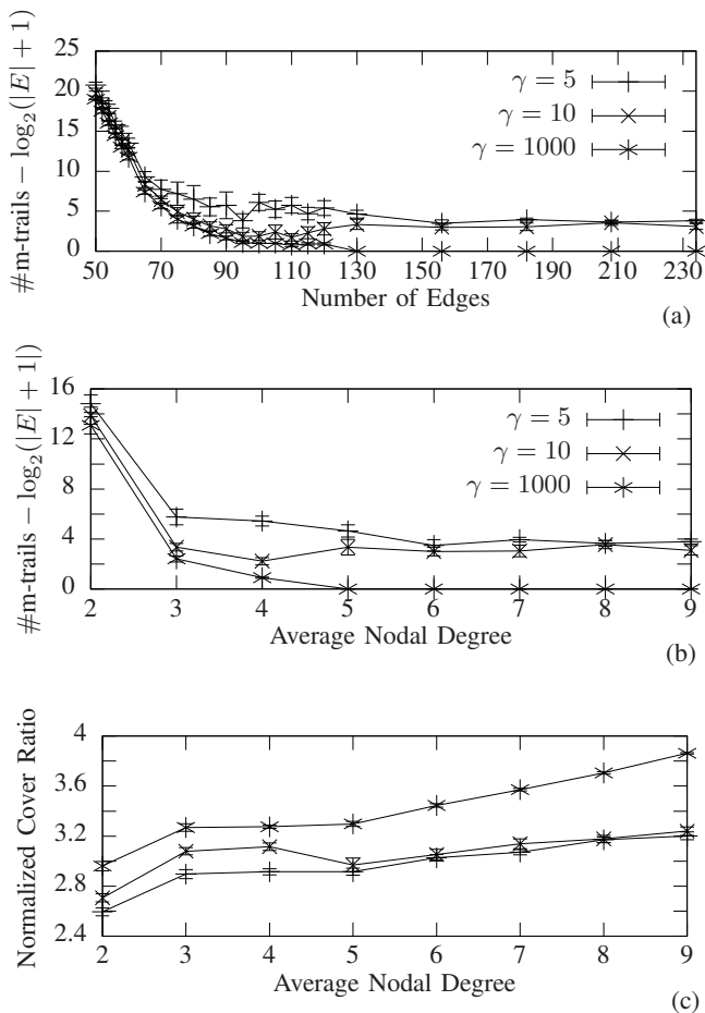
Fig. 9. Simulation on topologies with 50 nodes. (a), (b): normalized length of alarm code versus number of links (or the average nodal degree); and (c): normalized cover ratio versus average nodal degree.
