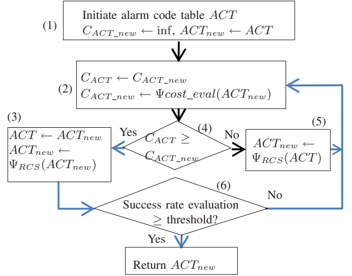
Fig. 5. The flowchart for the proposed heuristic algorithm.
