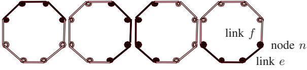
Fig. 3. Optimal M-trail assignment of an 8-node cycle.
