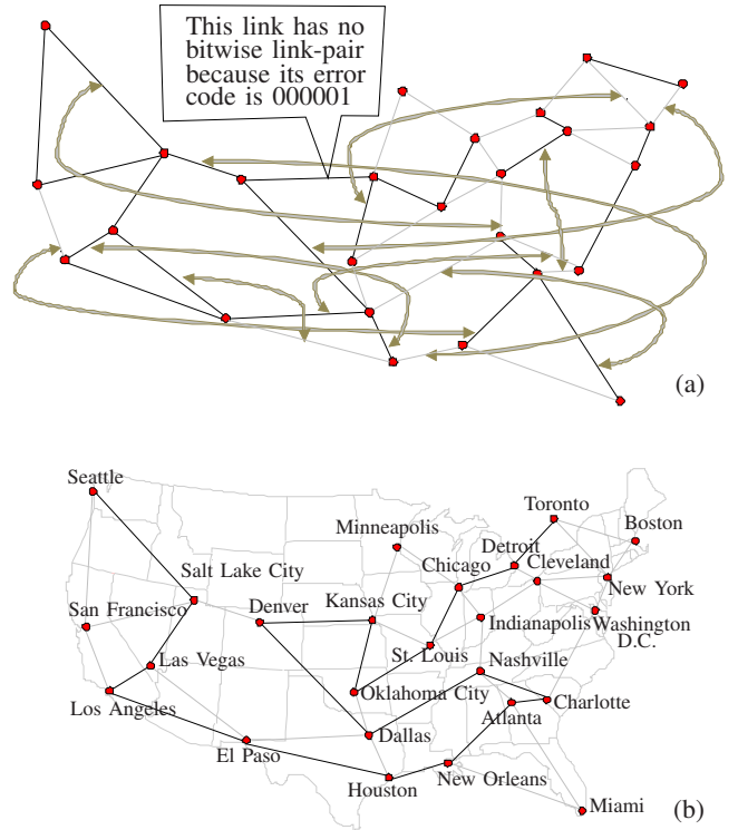
Fig. 7. Link set 6 (a) after random coding (b) after greedy random code swapping for link set 6 in the ACT.
