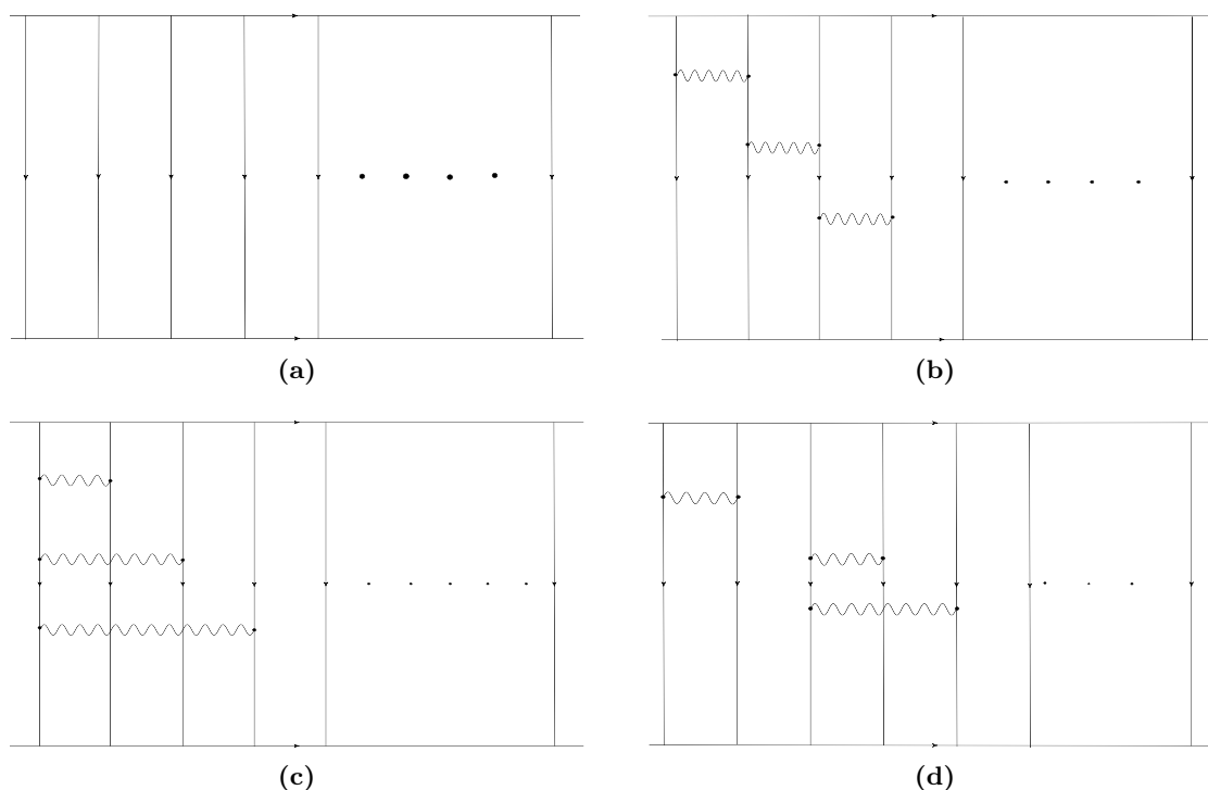
Figure 1. Some of the diagrams contributing to the energy of the lowest flux state, which is related to the dimension of the leading monopole operator.
