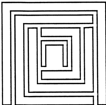
Figure 5.3. Depth k disassembly required.
