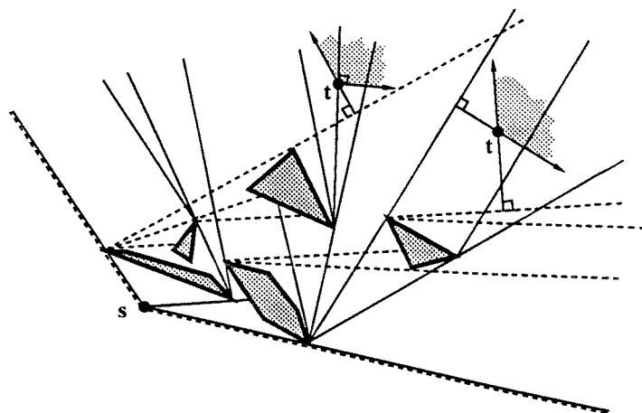
Figure 4.3. Example of a monotone path map.
