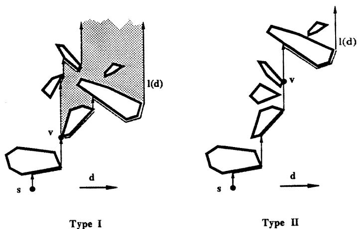
Figure 4.4. Events for sweeping l(d) .
