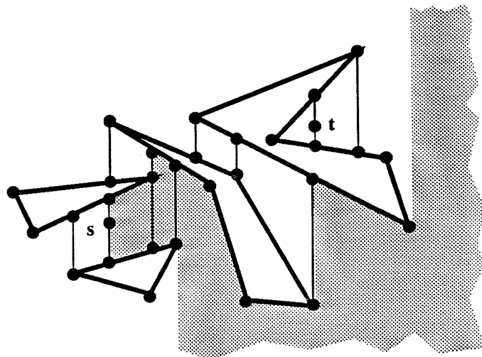
Figure 2.1. A vertical adjacency graph.
