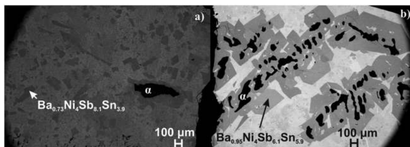
Fig. 10 Microstructure of the slowly cooled reguli used to grow the single crystals from the (a) (SnSb)-flux and (b) (Sn)-flux ( \alpha denotes the continuous solid solution of NiSb–Ni 3 Sn 2 ).
