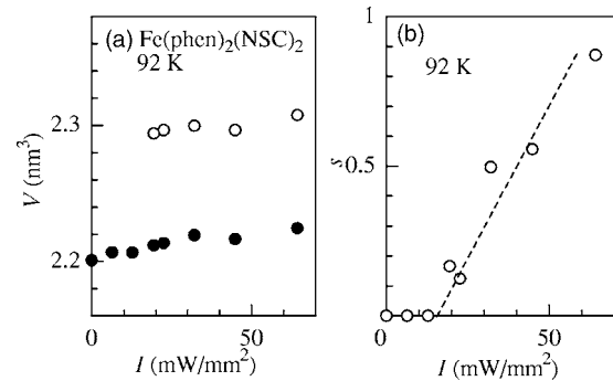
FIG. 3. (a) Cell volume ( V ) of \text{Fe}(\text{phen})_2(\text{NCS})_2 at 92 K against excitation power density ( I ). Closed and open circles stand for the LS phase and the on phase, respectively. (b) Mass fraction ( s ) of the on phase against I . A broken straight line is merely the guide for the eyes.
