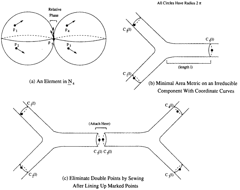
Fig. 1. The Morphisms and Minimal Area Metrics.
