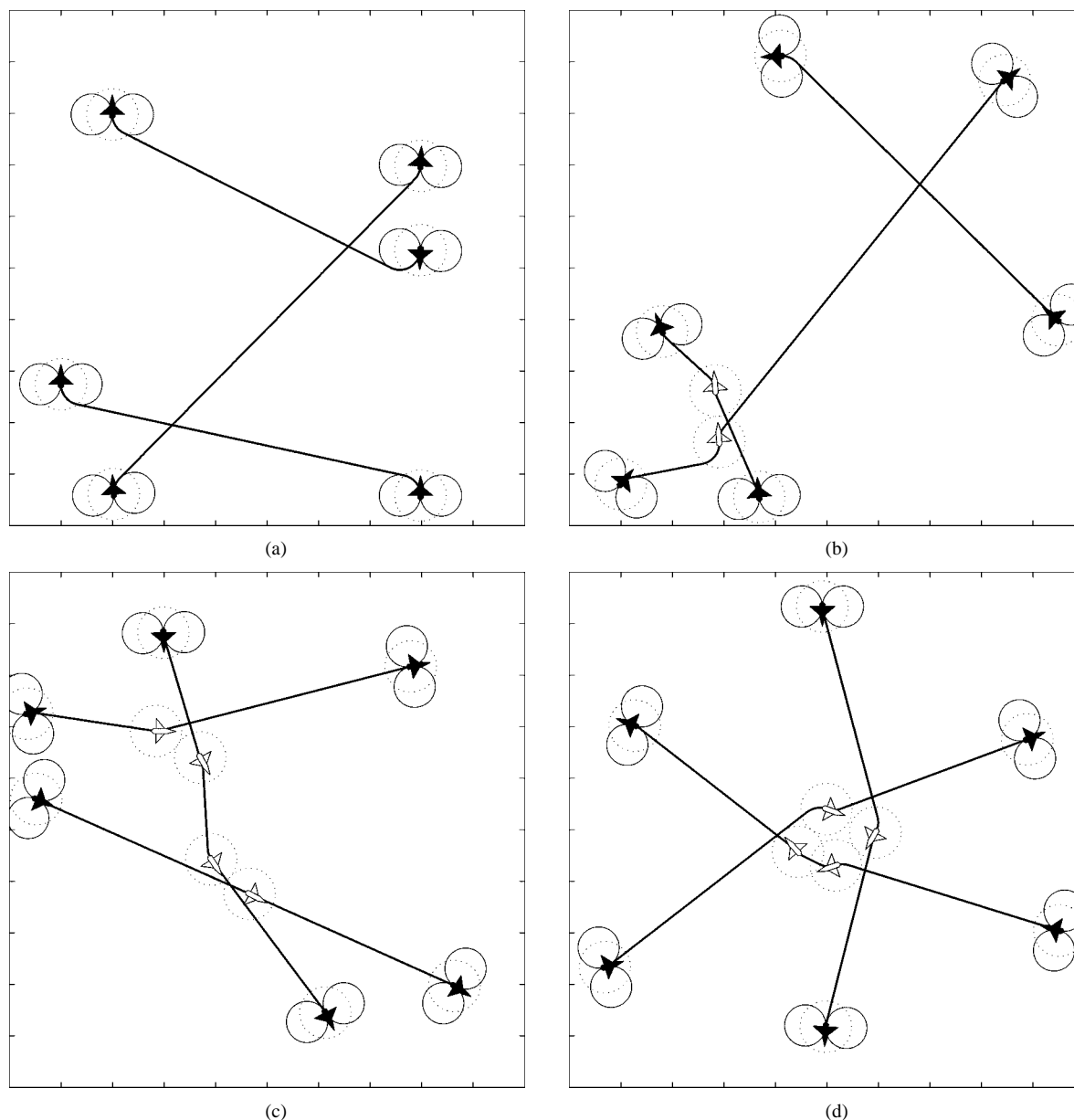
Fig. 7. Four cases of three-aircraft conflict resolution. (a) Conflict is resolved at level 0. (b) Level 1 solution. (c) Level 2 solution. (d) Level 2 resolution that generates a roundabout-like maneuver.
