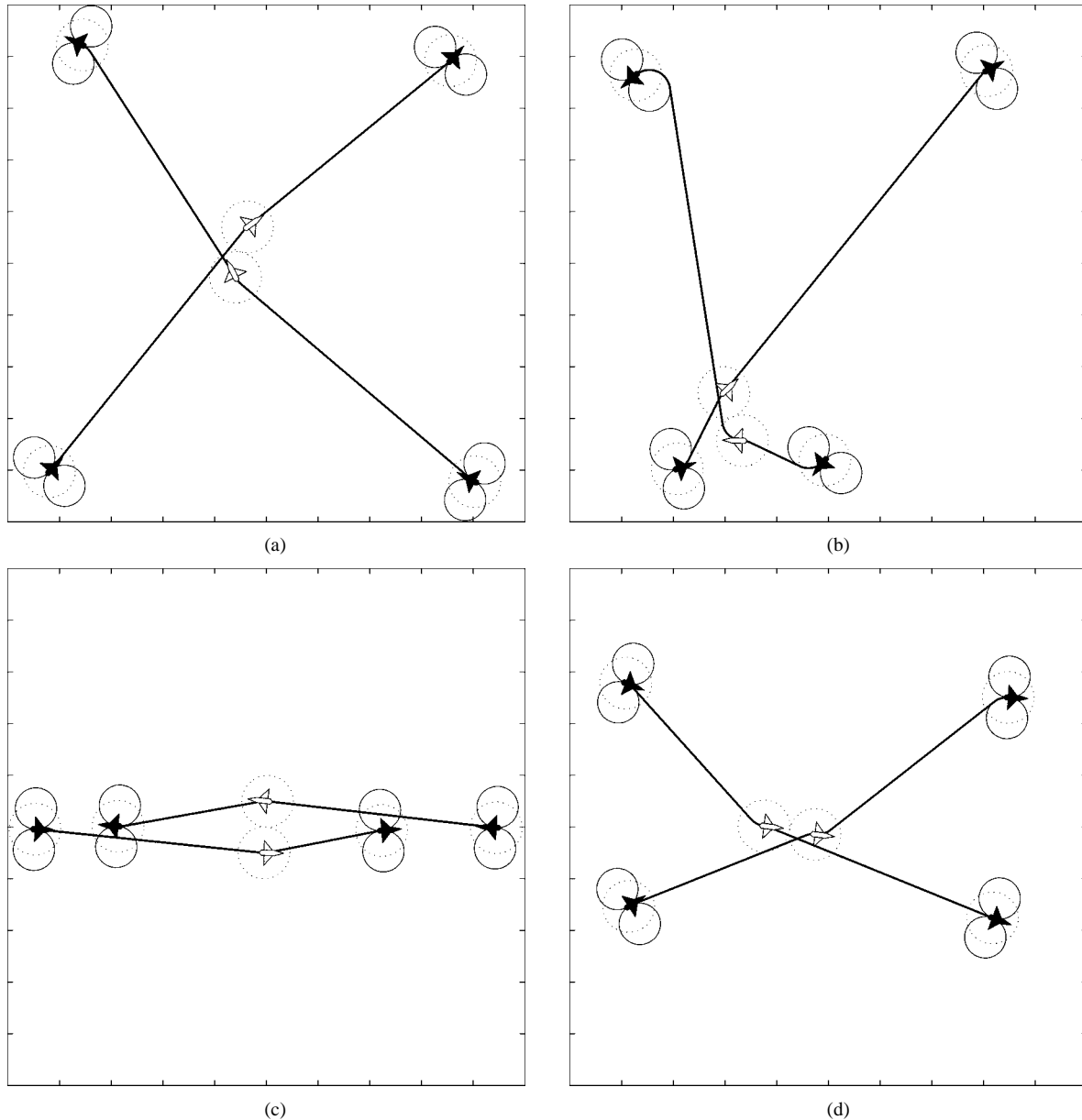
Fig. 6. Numerically computed solutions to optimal cooperative conflict resolution for two aircraft. Minimum curvature circles are reported at the start and goal configurations, along with safety discs of radius d/2 (dashed).
