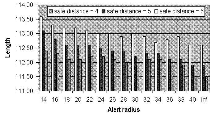
Fig. 10. Total length flown by aircraft at varying the alert zone radius. The measures are in nautical miles.
