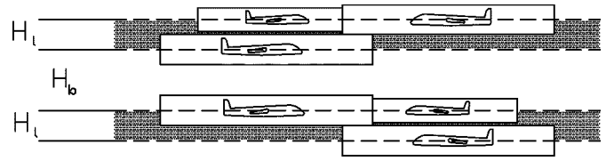
Fig. 2. The airspace is structured in separate layers within which traffic conflicts have to be resolved.
