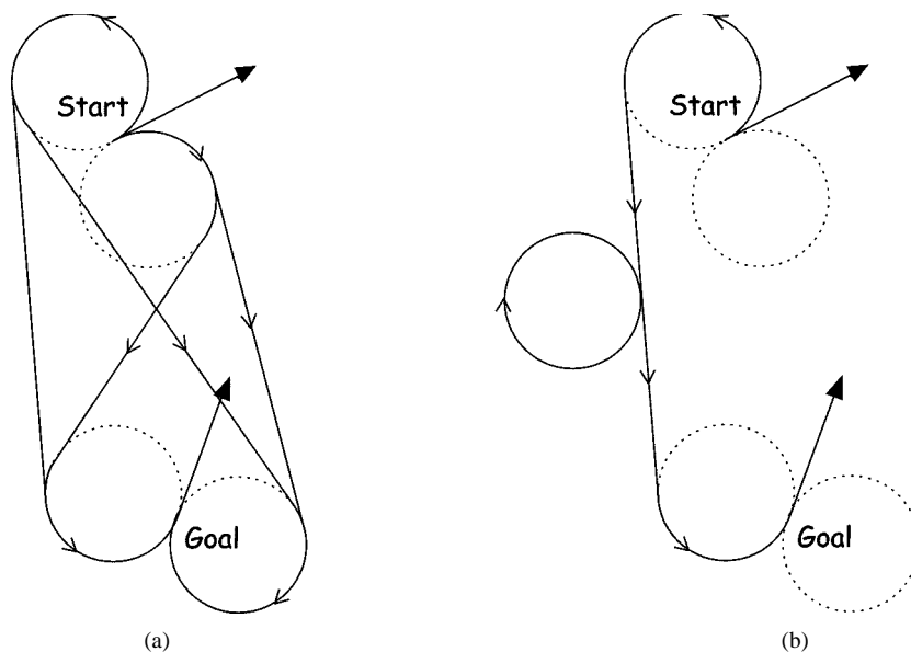
Fig. 3. (a) Four extremal arcs of type CSC joining two waypoints. (b) Extremal arc for the same waypoints including a “waiting” circle.
