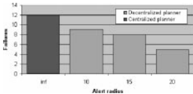
Fig. 11. Fault tolerance to controller failures at varying the degree of decentralization. The number of accidents is relative to 100 crisis situations. Labels on the x axis refer to alert radii measured in nautical miles.
