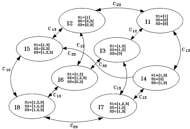
Fig. 8. A decentralized ATMS with three aircraft having equal alert radius. Each node in the graph corresponds to different costs and constraints in the agents' optimal steering problem. Optimizing controllers for such problems cause different continuous time dynamics at each node. Switching between modes is triggered when an airplane enters or exits the alert neighborhood of another ( D_{i,j} changes sign).
