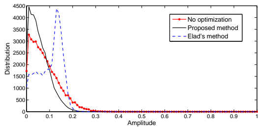
(b) \Phi : Random, and \Psi : DCT.
