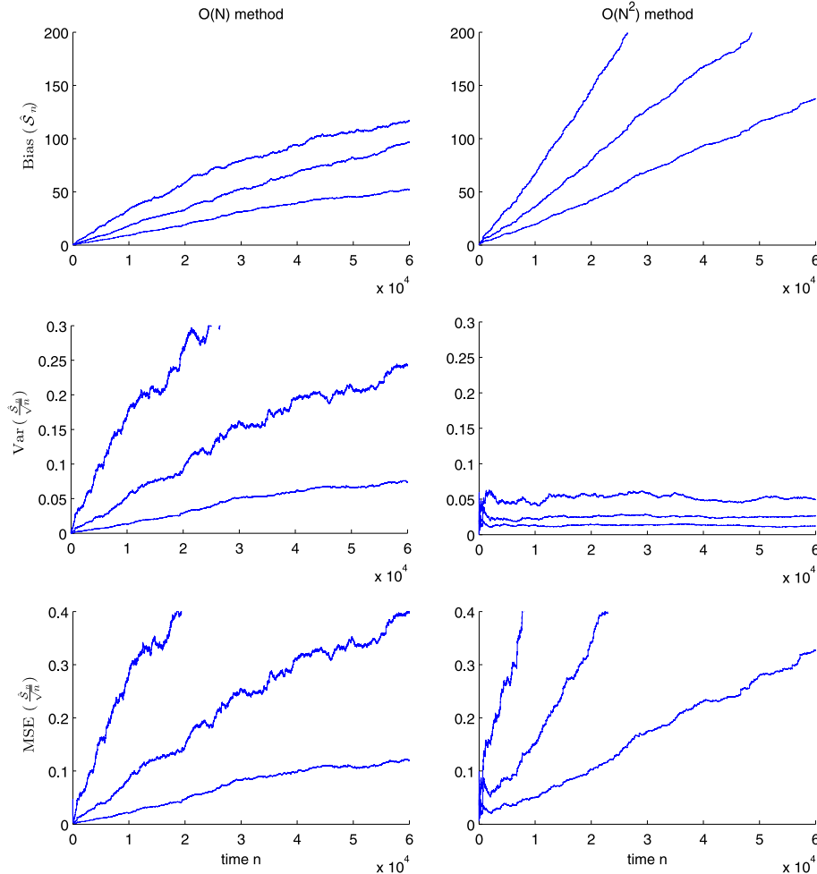
FIG. 1. Estimating smoothed additive functionals: empirical bias of the estimate of S_n^\theta (top panel), empirical variance (middle panel) and MSE (bottom panel) for the estimate of S_n^\theta/\sqrt{n} . Left column: \mathcal{O}(N) method using N^2 = 2500, 10,000, 40,000 particles. Right column: \mathcal{O}(N^2) method using N = 50, 100, 200 particles. In every subplot, the top line corresponds to using N = 50 , the middle for N = 100 and the lower for N = 200 .
