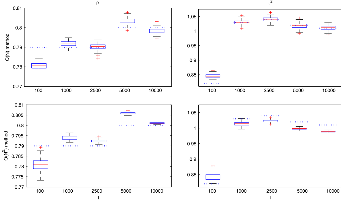
FIG. 2. Off-line EM: boxplots of \hat{\theta}_n for various T using 25 iterations of off-line EM and 150 realizations of the algorithms. Top panels: \mathcal{O}(N) method using N = 150^2 particles. Bottom panels: \mathcal{O}(N^2) with N = 150 . The dotted horizontal lines are the ML estimate for each time T obtained using Kalman filtering on a grid.
