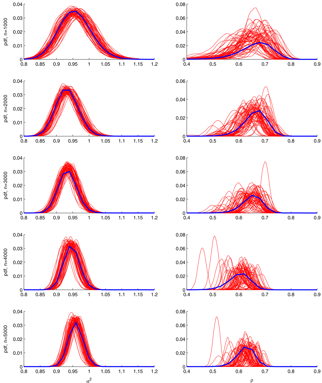
FIG. 5. Particle method with MCMC steps, \theta = (\rho, \sigma^2) ; estimated marginal posterior densities for n = 10^3, 2 \times 10^3, \dots, 5 \times 10^3 over 50 runs (red) versus ground truth (blue).
