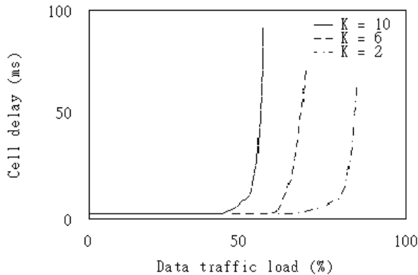
Figure 7. Cell delay characteristics of transmitted data
