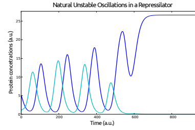
Fig. 2. Natural oscillatory behaviour of a generalised repressilator system consisting of 6 genes. The blue line represents the time evolution of the protein concentration produced by the expression of gene 1; the cyan line represents the time evolution of the protein concentration produced by the expression of gene 2. The oscillations have a period of approximately 150 arbitrary time units but are, however, not stable.
