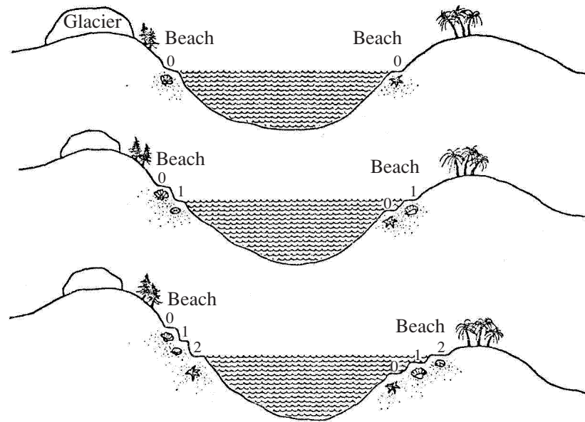
Figure 1. Schematic illustration of sea-level changes on a viscoelastic earth model, taken from Farrell & Clark (1976, Fig. 6).
