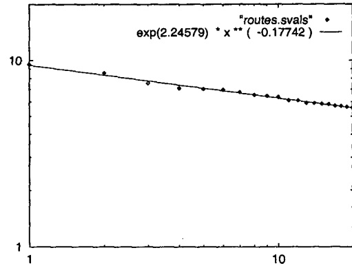
(b) Rout-95
