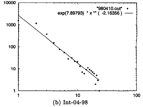
Figure 5: The outdegree plots: Log-log plot of frequency f_d versus the outdegree d .
