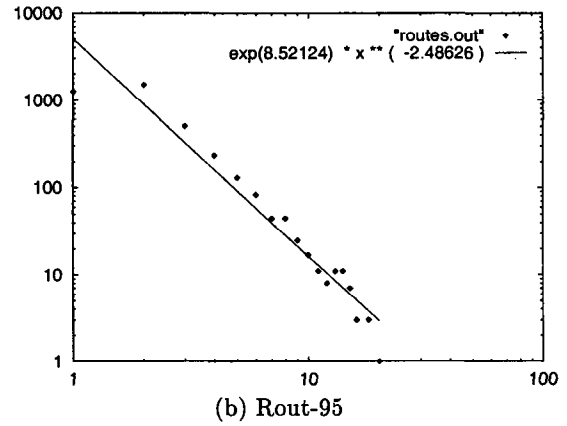
Figure 6: The outdegree plots: Log-log plot of frequency f_d versus the outdegree d .
