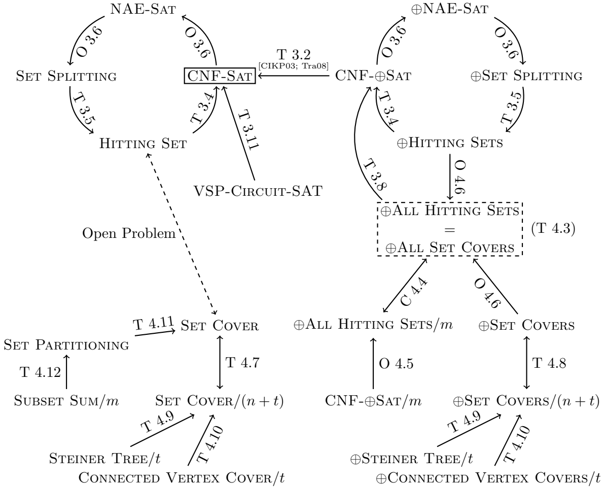
Figure 1: Overview of the reduction graph in this paper. An arrow \Pi'/s' \rightarrow \Pi/s depicts a reduction from the problem \Pi' to the problem \Pi with the following implication: If \Pi can be solved in time c^s \cdot \text{poly} , then \Pi' can be solved in time c^{s'} \cdot \text{poly} . The edge labels depict the theorem (T), corollary (C), or observation (O) that contains the formal statement of the reduction. When the size parameter s is the number of vertices or variables n , we omit it. Other parameters are: the number m of clauses, hyperedges, or the number of bits used to represent the input integers in SUBSET SUM; and the size t of the solution that we are looking for. Note that the figure suppresses details about which reductions require or preserve that the instances have bounded clause or hyperedge width, or bounded density. On the left, we have decision problems, and on the right we have parity problems; the two groups are related via the isolation lemma [CIKP03; Tra08], cf. Theorem 3.2. Furthermore, we observe a cluster on the top, which contains problems for which the best-known algorithm is naïve brute force; see Section 3. And there is a cluster on the bottom, which contains problems for which the best-known algorithm has a dynamic programming flavor; see Section 4. These two clusters are connected in the parity world via our “flip theorem”, Theorem 4.3. In the decision world, this connection is an open problem: Does SETH imply the assumption of Theorem 1.2?
