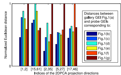
Fig. 4. Normalized Euclidean distances from gallery sample Fig. 1a to probe samples Figs. 1b, 1c, 1d, 1e, 1f, 1g, based on different projection directions.
