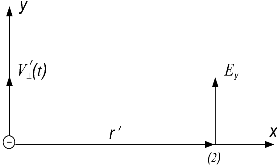
Fig. 4. Formation of the retarded scalar-vector potential.
