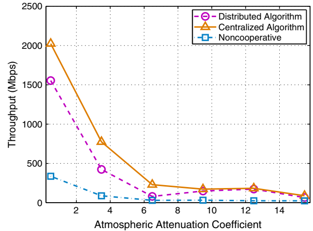
Fig. 5 Throughput versus attenuation coefficient \alpha
