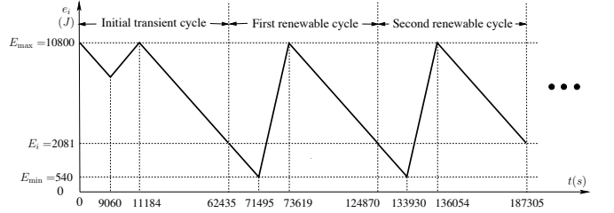
Fig. 8. The energy behavior of the bottleneck node (the 38th node) in the 50-node network. Traveling direction is counter clockwise.
