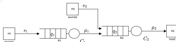
Figure 1: Prototype network with two buffers.
