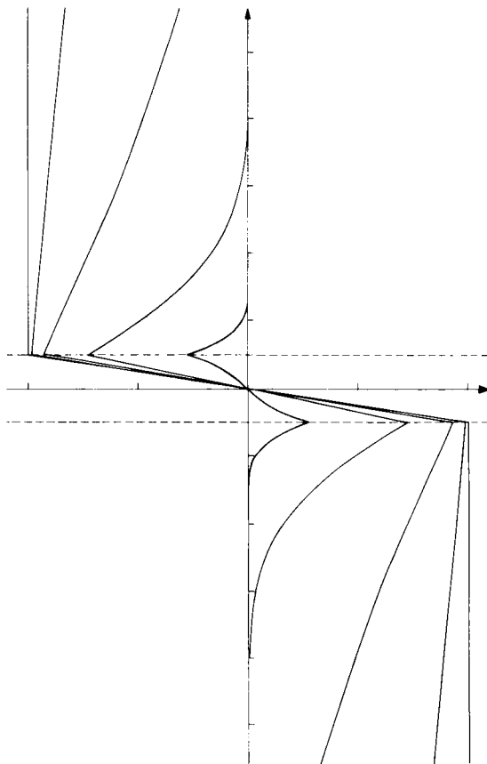
FIG. 2. Instantaneous distributions of secondary vorticity associated with the first internal mode on a thin, deep thermocline occupying the region \frac{1}{2}b > z > -\frac{1}{2}b .
