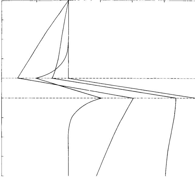
FIG. 1. Instantaneous distributions of secondary vorticity associated with the first internal mode on a thin, shallow thermocline occupying the region -4b > z > -5b .
