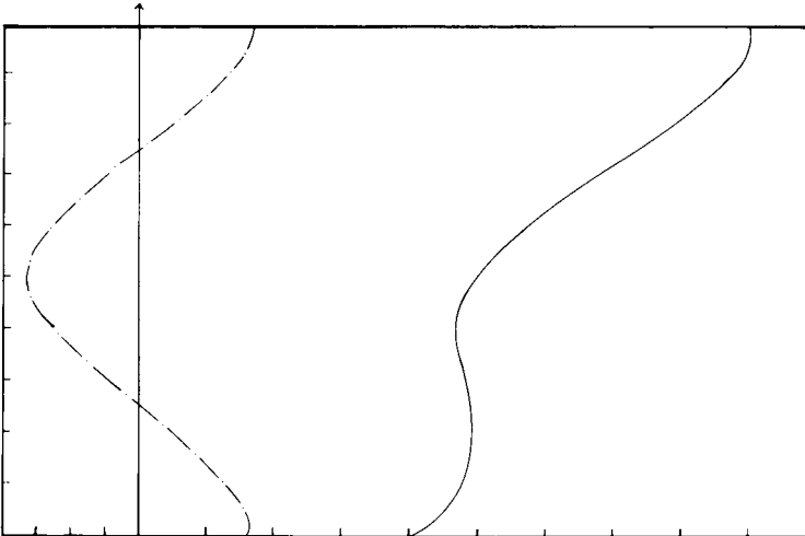
FIG. 3. Profiles of the mass transport velocity (—) and the Stokes drift velocity (---) for the first internal mode in a uniformly-stratified fluid.
