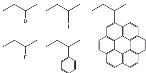
Figure 2. Series of substituted 2-butanenes. (Reproduced from Ref. [21], with permission).
