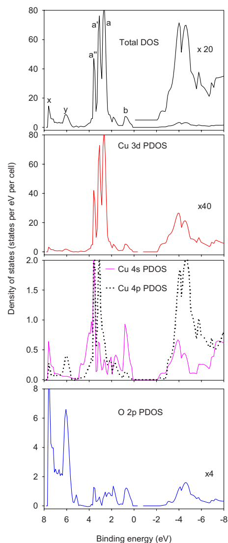
FIG. 1. (Color online) Full and partial densities of states for Cu 2 O derived from band structure calculations.
